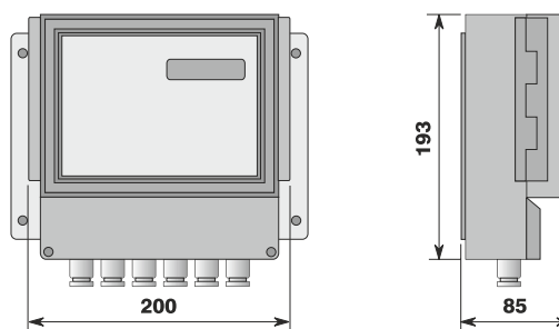
ELECTRONIC UNIT
